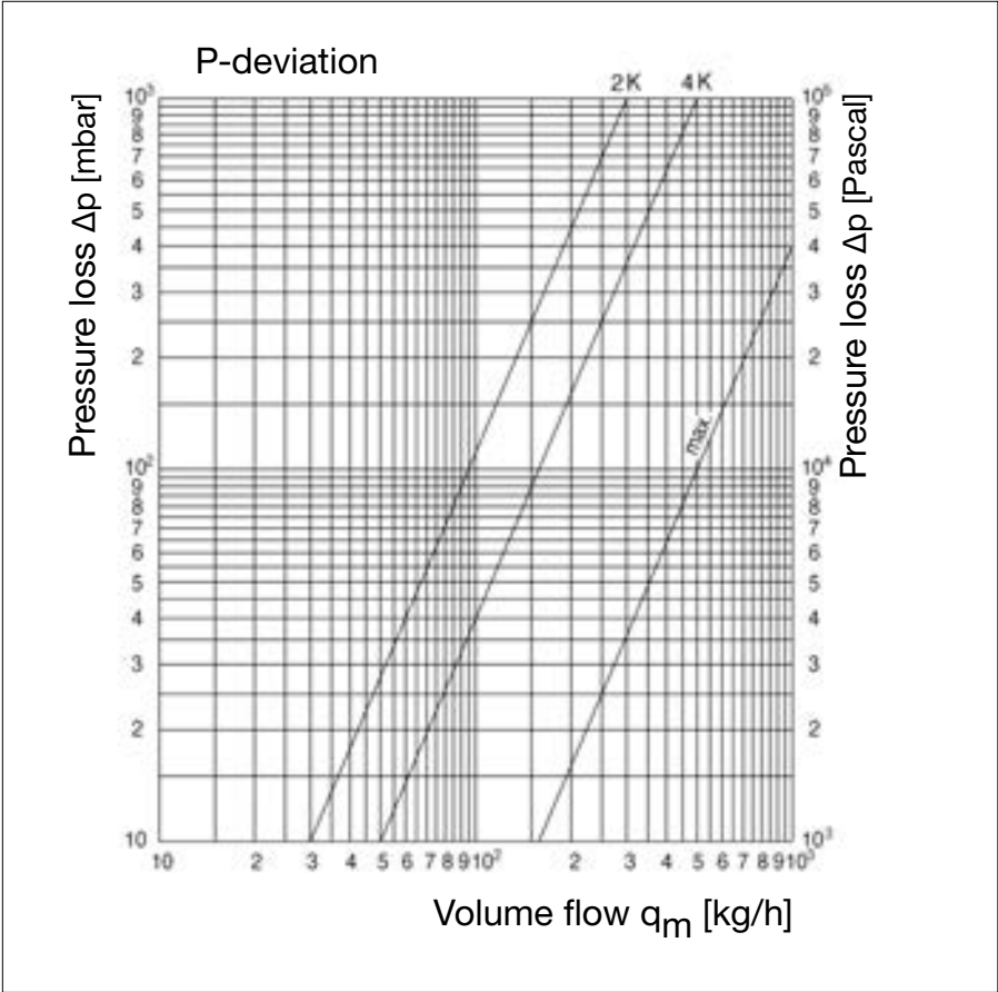
Pressure loss diagram for Schlüter®-BEKOTEC-THERM-RTB 4K P deviation; factory default setting
